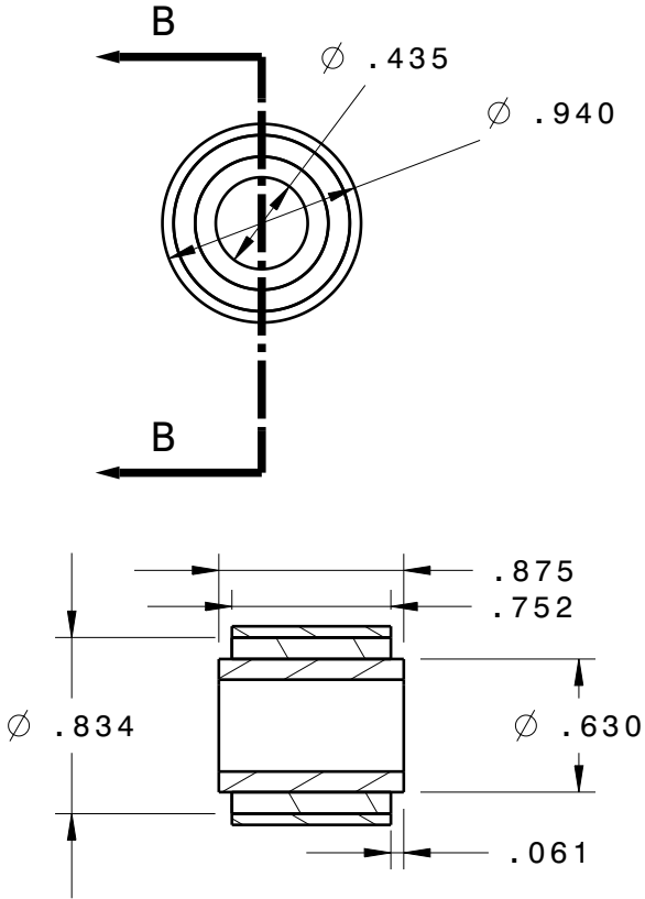
Gear Lever Bushing Section view B-B
